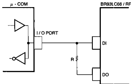
Fig.11 Common connections for the DI and DO control line
