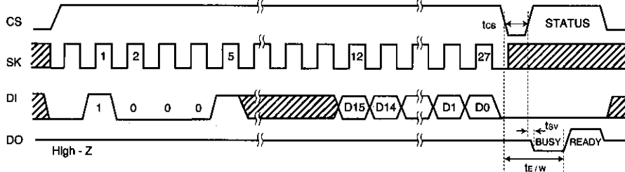
Fig.5 All address write cycle timing
