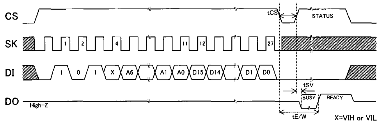
Fig.-13 Write Cycle Timing
