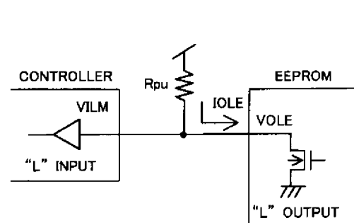
Fig.6-3 PULL UP RESISTER OF DO PIN
