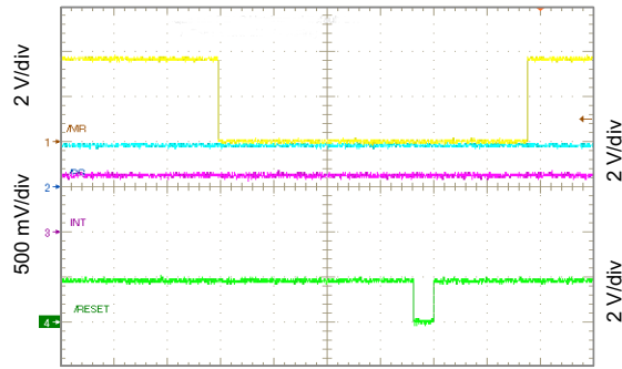
Figure 101. \overline{\text{RESET}} Timing
