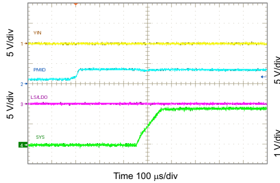
Figure 38. Battery Connected to V_{(BAT)}
