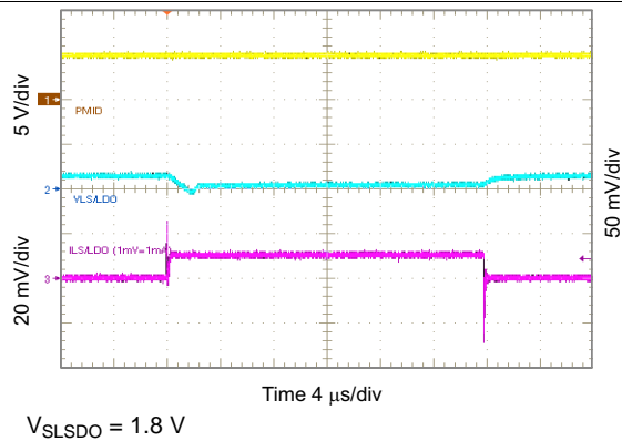
Figure 85. 1.8 V LSLDO Load Transient, 0 to 10 mA
