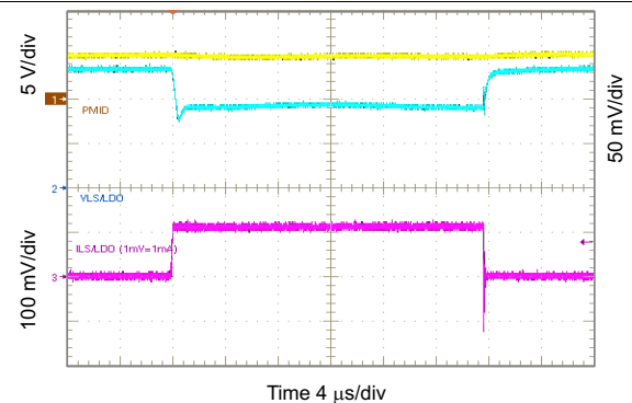
Figure 90. 1.8 V_{SLSDO} Load Transient, 0 to 100 mA
