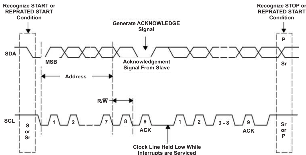
Figure 9. Bus Protocol
