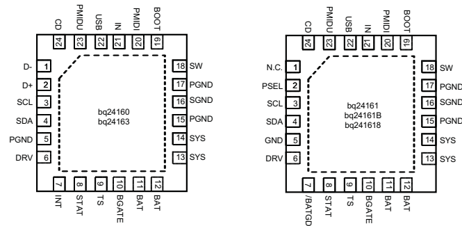
Figure 1. 24-Pin QFN (RGE)
