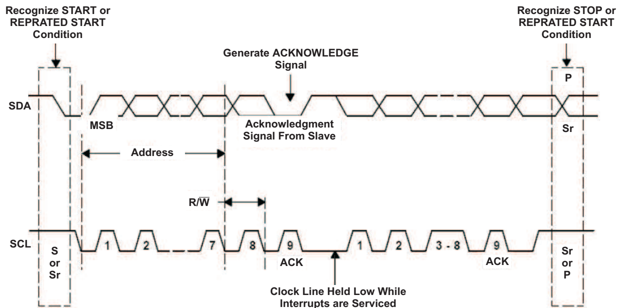
Figure 31. Bus Protocol
