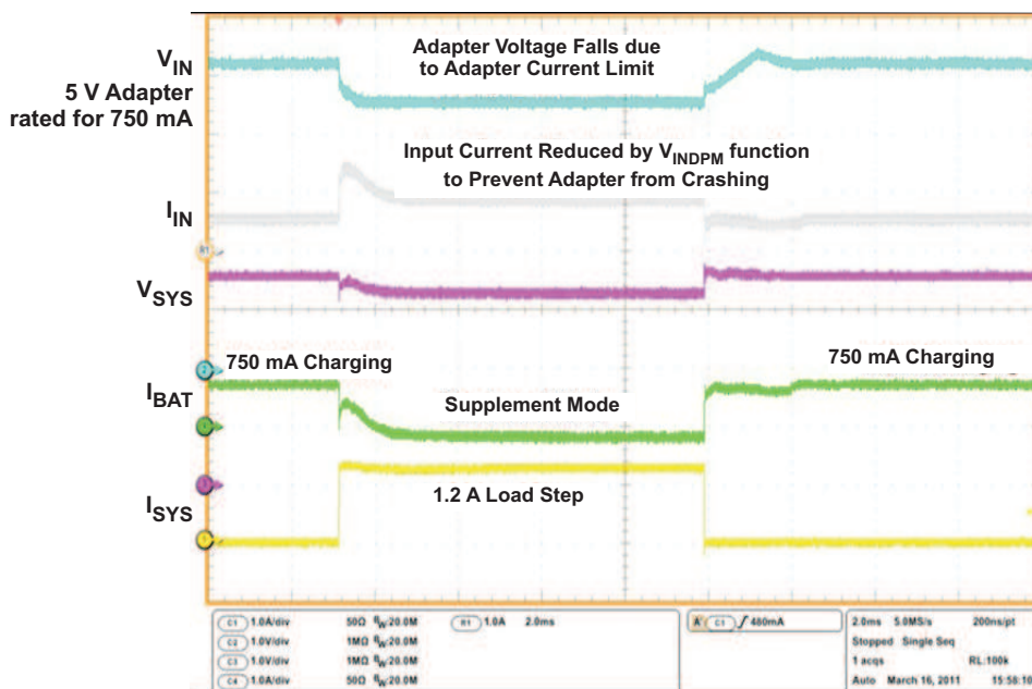
Figure 27. bq24160 V IN -DPM
