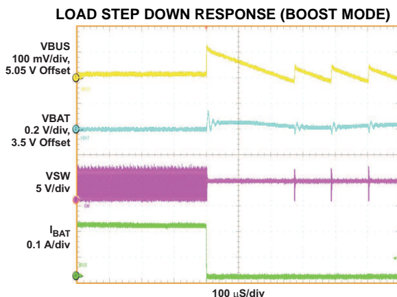
Figure 19. VBUS = 5.05 V, V BAT = 3.5V, I BUS = 217 mA
