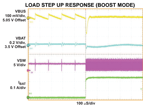
Figure 18. VBUS = 5.05 V, V BAT = 3.5V, I BUS = 0-217 mA
