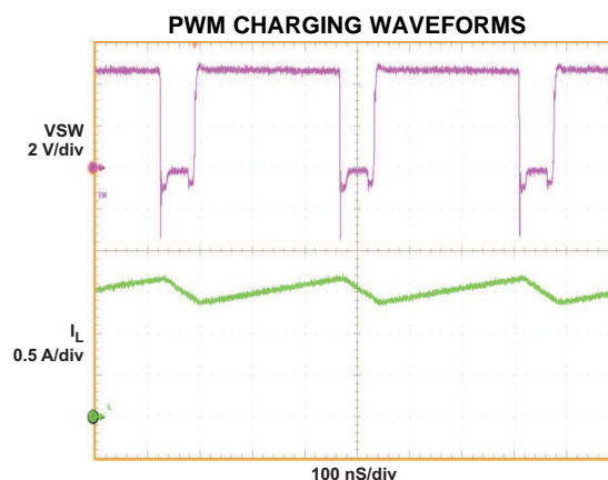
Figure 7. \text{VBUS} = 5\text{V} , \text{V}_{\text{BAT}} = 2.6\text{V} , \text{Vreg} = 4.2\text{V} , \text{I}_{\text{CHG}} = 1550\text{mA}
