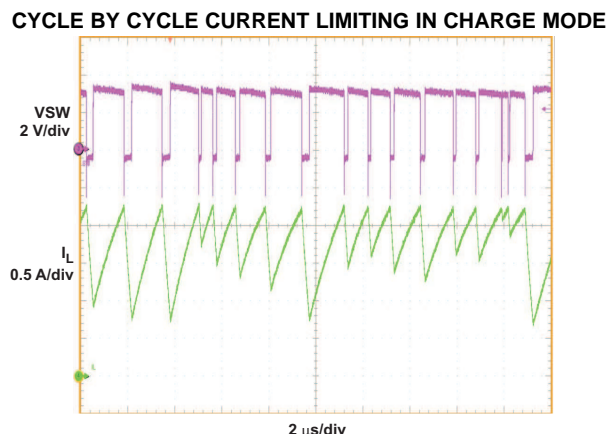
Figure 5. \text{VBUS} = 5\text{V} , \text{V}_{\text{BAT}} = 3.5\text{V} Charge Mode Overload Operation
