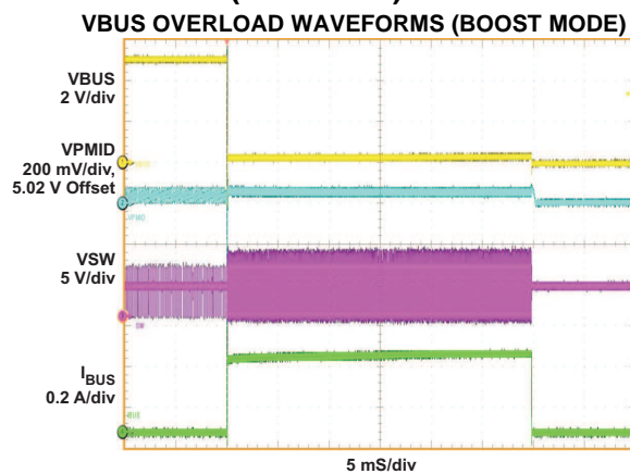
Figure 17. VBUS = 5.05 V, V BAT = 3.5V, R LOAD (at VBUS) = 1k \Omega to 0.5 \Omega
