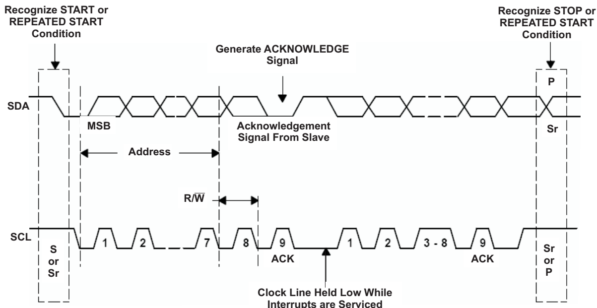
Figure 34. Bus Protocol
