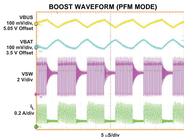
Figure 16. VBUS = 5.05 V, V BAT = 3.5V, I BUS = 42 mA
