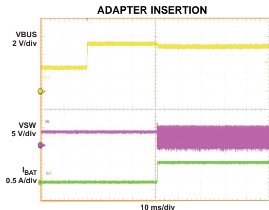
Figure 4. \text{VBUS} = 0\text{--}5\text{V} , \text{lin\_limit} = 500\text{mA} , \text{Vreg} = 4.2\text{V} \text{VBAT} = 3.5\text{V} , \text{I}_{\text{CHG}} = 550\text{mA} , 32S mode
