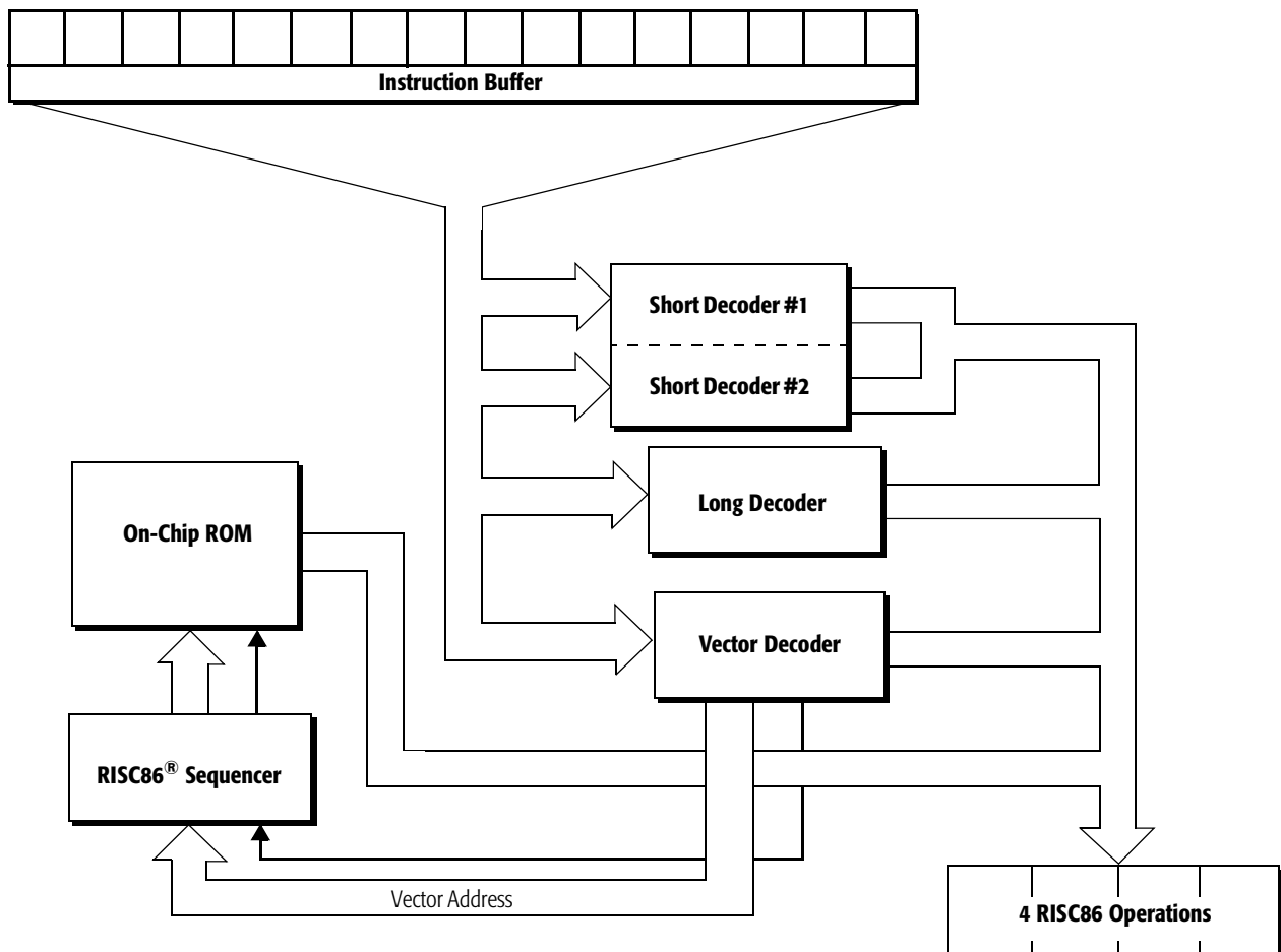
Figure 4. Mobile AMD-K6 ® -III-P Processor Decode Logic
