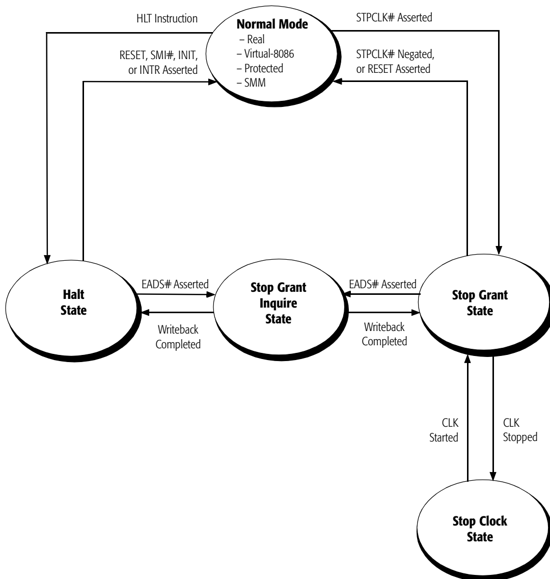
Figure 7. Clock Control State Transitions
