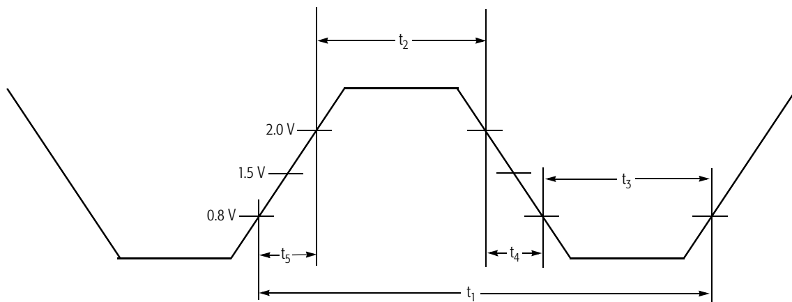
Figure 9. CLK Waveform
