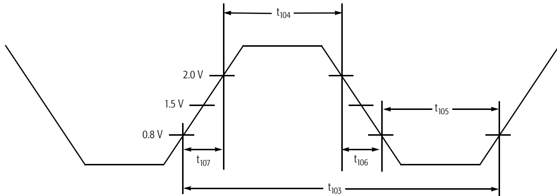
Figure 15. TCK Waveform
