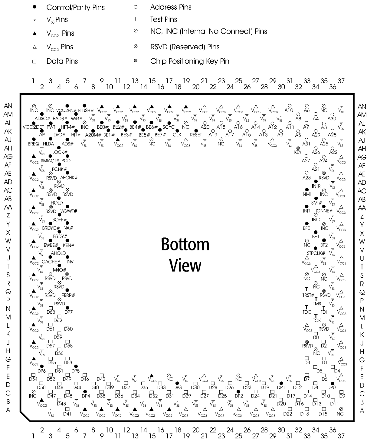
Figure 24. Mobile AMD-K6®-III-P Processor Bottom-Side View
