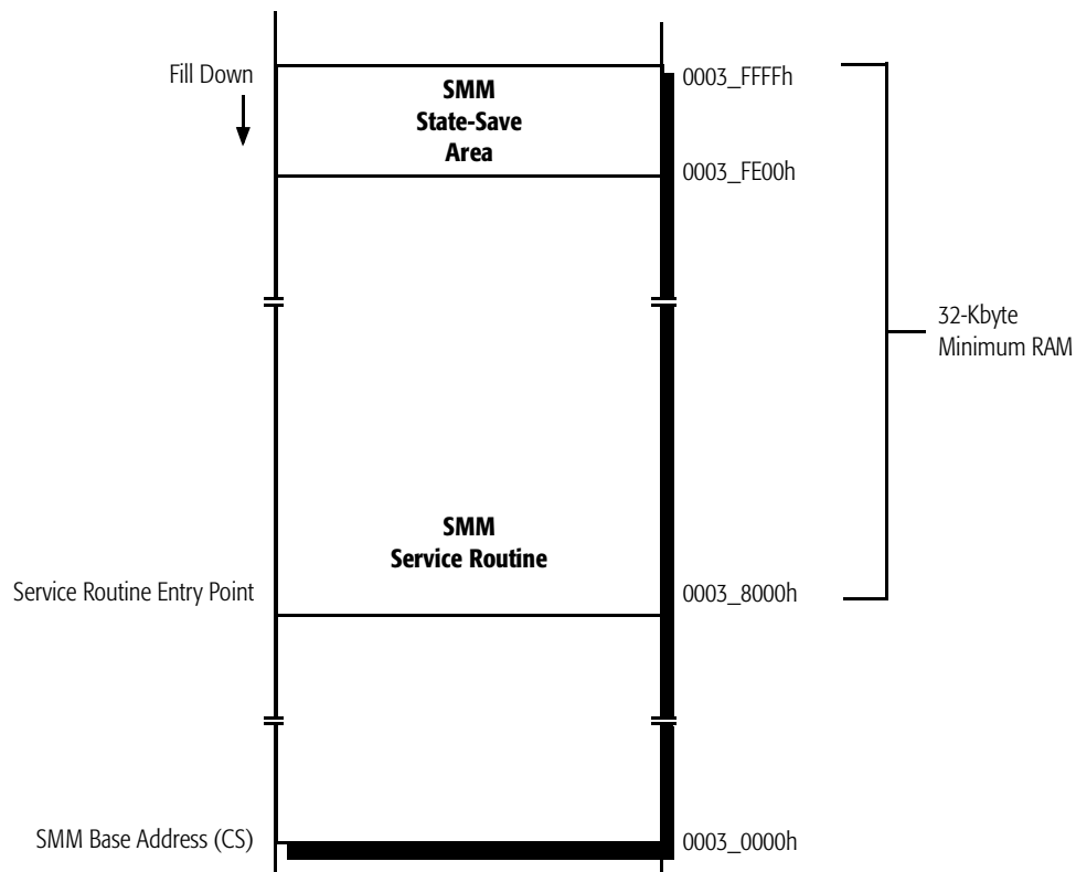
Figure 8. SMM Memory
