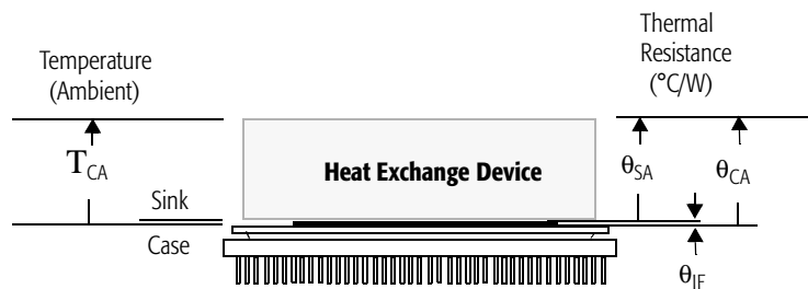
Figure 19. Thermal Model
