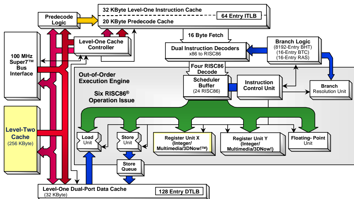
Figure 1. Mobile AMD-K6®-III-P Processor Block Diagram
