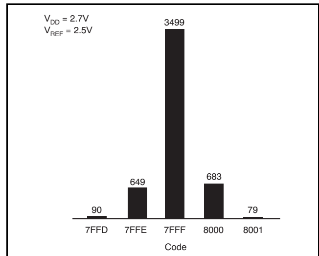
Figure 35. 5000 Conversion Histogram of a DC Input
