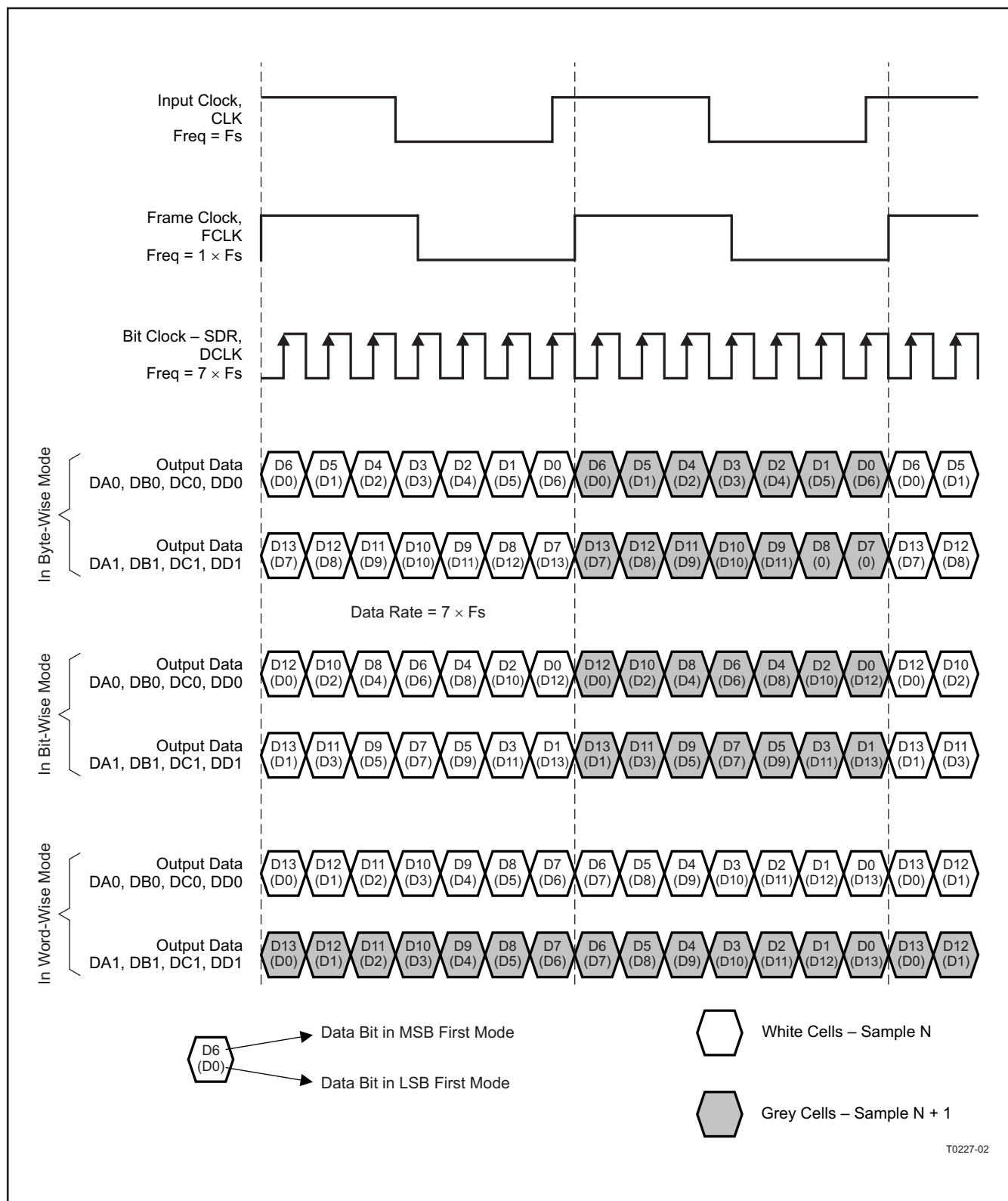
Figure 96. 2-Wire Interface 14× Serialization - SDR Bit Clock
