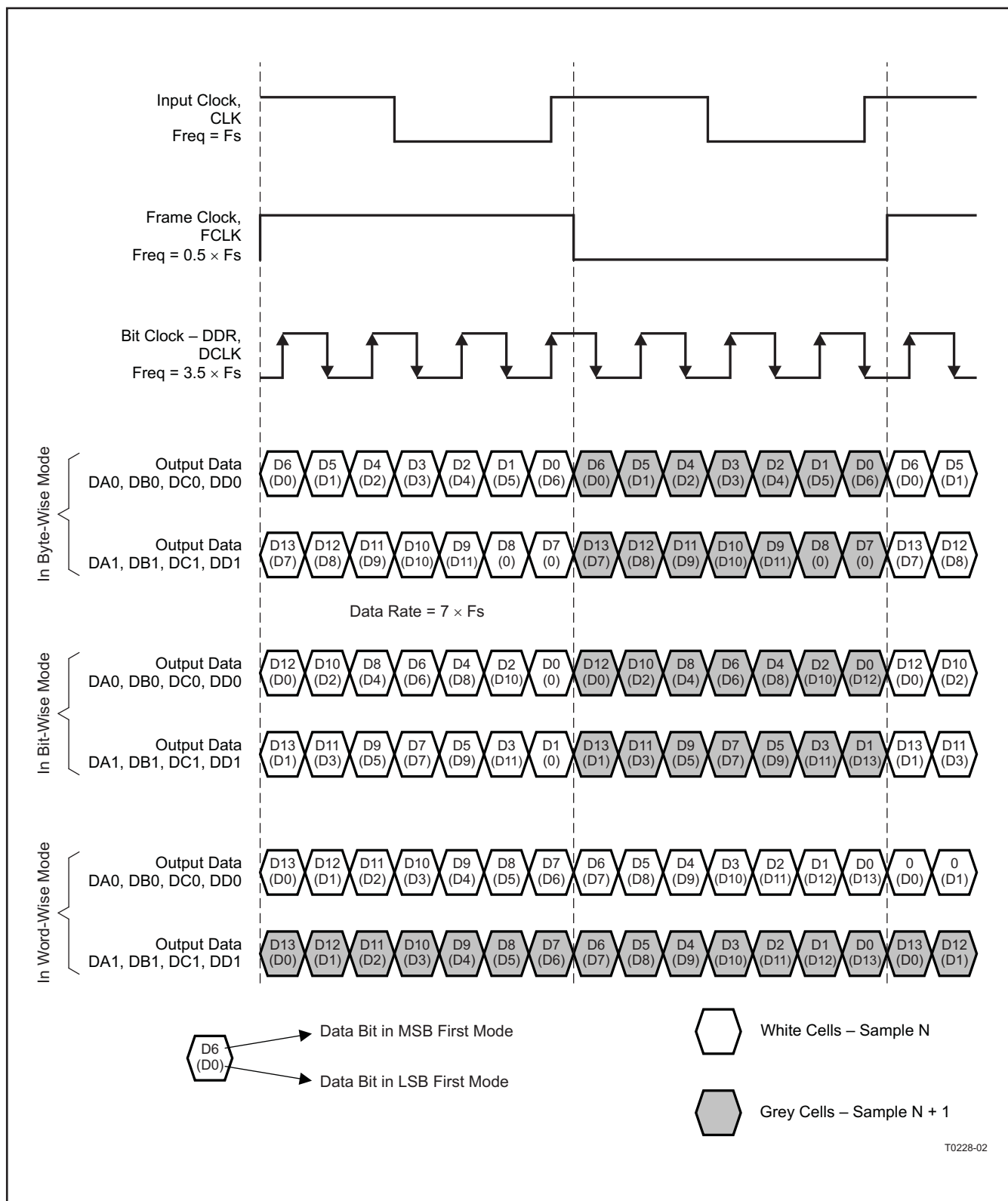
Figure 97. 2-Wire interface 14× Serialization - DDR Bit Clock
