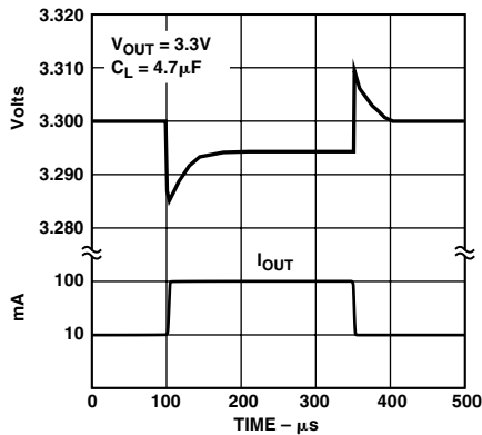
TPC 13. Load Transient
