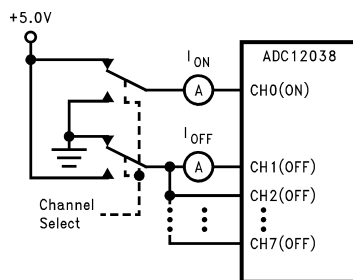
Figure 11. Leakage Current
