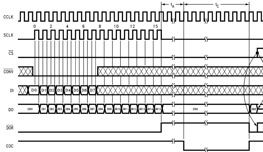
Figure 24. ADC12038 Software Power Up/Down Using \overline{\text{CS}} with 16-Bit Digital Output Format
