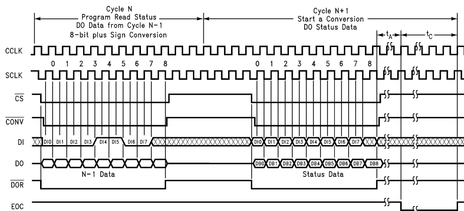
Figure 27. ADC12038 Configuration Modification—Example of a Status Read
