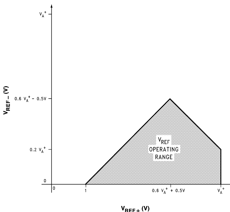
Figure 40. V_{REF} Operating Range
