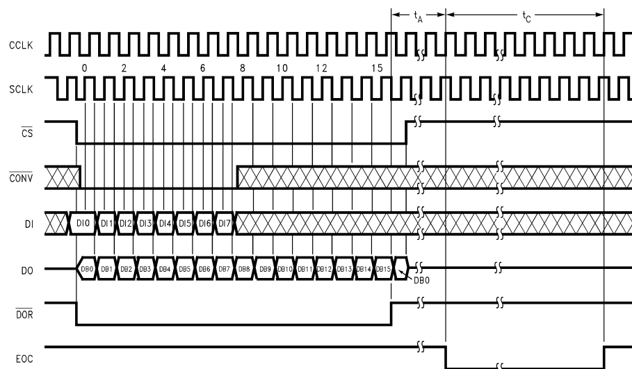
Figure 21. ADC12038 Conversion Using \overline{\text{CS}} with 16-Bit Digital Output Format
