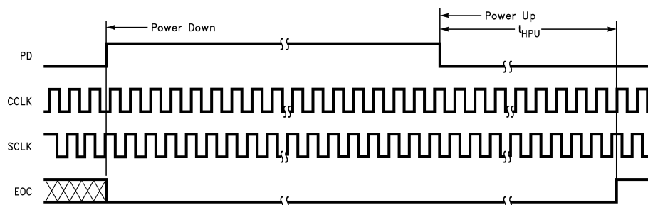
Figure 26. ADC12038 Hardware Power Up/Down
