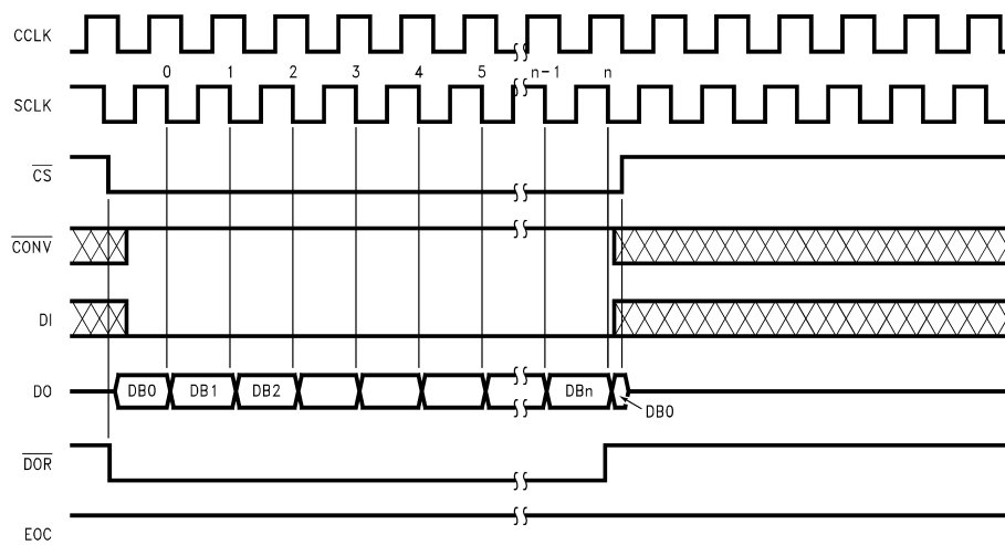
Figure 18. ADC12038 Read Data without Starting a Conversion Using \overline{\text{CS}}
