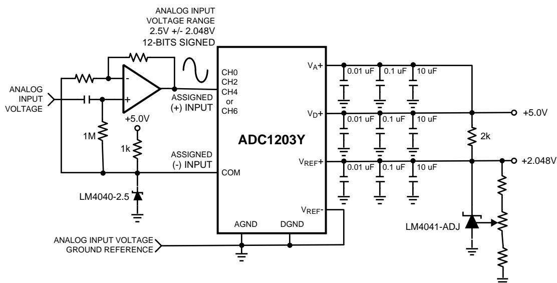
Figure 37. Pseudo-Differential Biasing without the Loss of Digital Output Range
