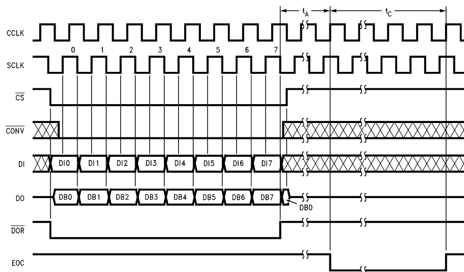
Figure 20. ADC12038 Conversion Using \overline{\text{CS}} with 8-Bit Digital Output Format
