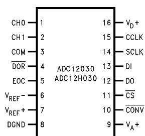
Figure 1. 16-Pin Wide Body SO Packages Top View
