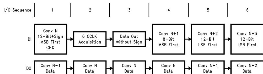
Figure 31. Changing the ADC's Conversion Configuration
