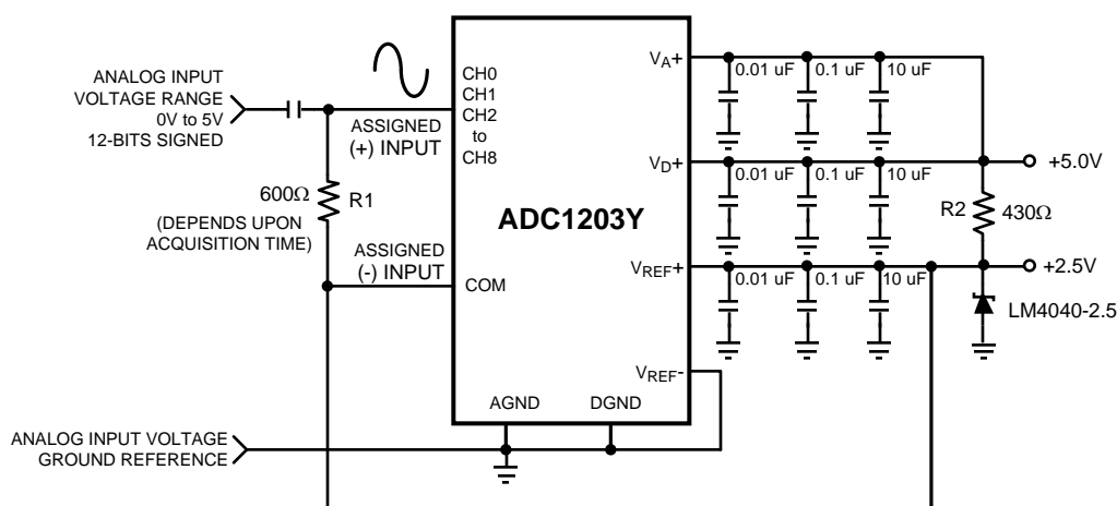
Figure 35. Pseudo-Differential Biasing with the Signal Source AC Coupled Directly into the ADC
