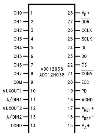
Figure 4. 28-Pin Wide Body SO Packages Top View
