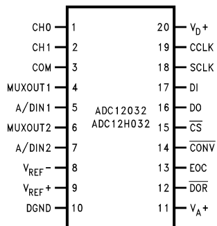
Figure 2. 20-Pin Wide Body SO Packages Top View
