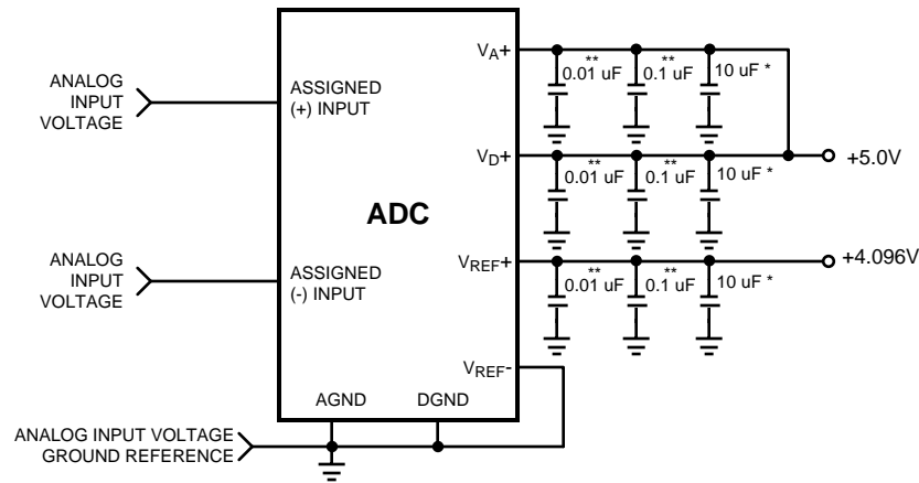
Figure 28. Recommended Power Supply Bypassing and Grounding
