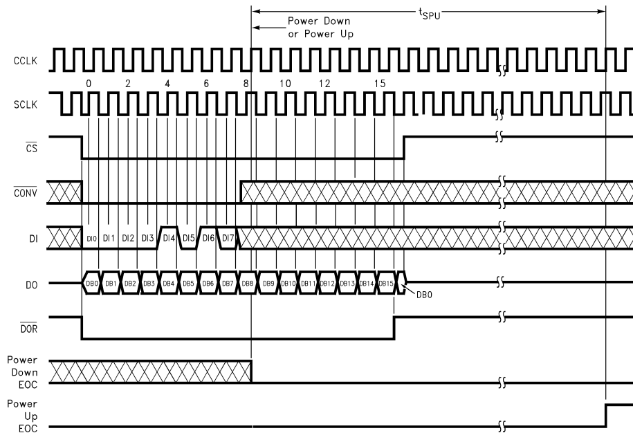
Figure 24. ADC12038 Software Power Up/Down Using \overline{\text{CS}} with 16-Bit Digital Output Format
