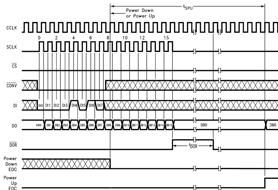
Figure 26. ADC12038 Hardware Power Up/Down
