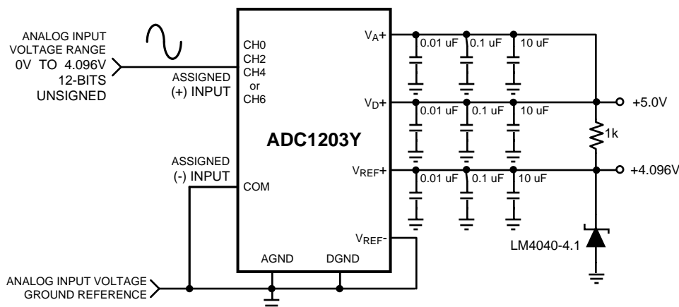
Figure 34. Single-Ended Biasing
