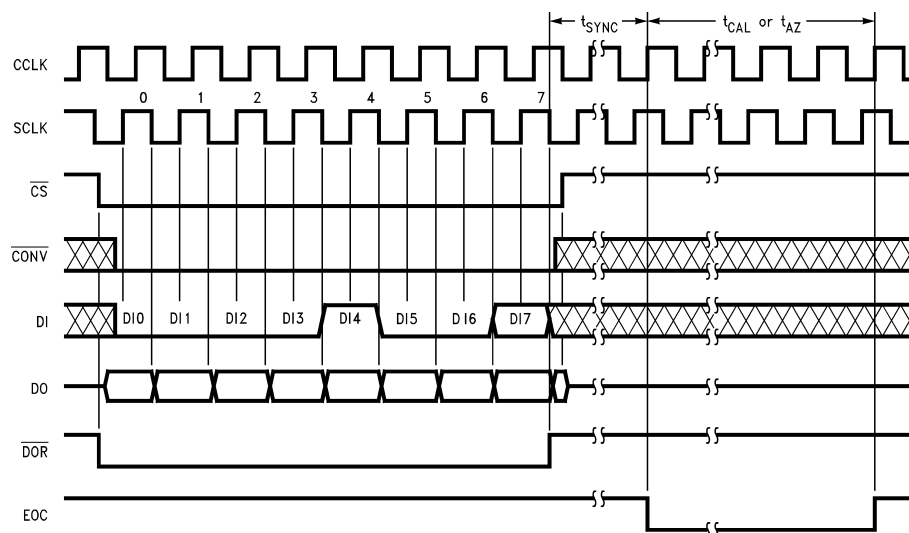
Figure 17. ADC12038 Auto Cal or Auto Zero
