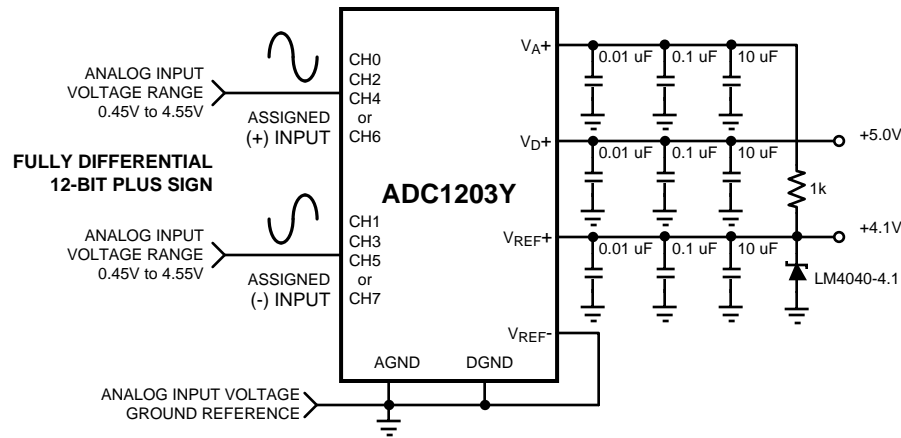
Figure 38. Fully Differential Biasing
