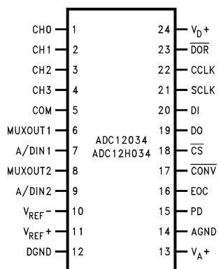
Figure 3. 24-Pin Wide Body SO, DIP, SSOP-EIAJ Packages Top View
