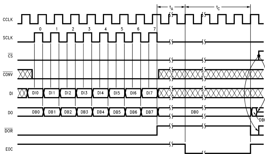
Figure 22. ADC12038 Conversion with \overline{\text{CS}} Continuously Low and 8-Bit Digital Output Format
