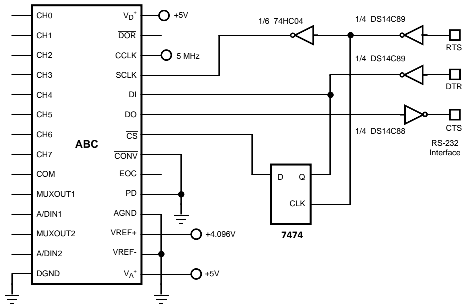
Figure 41. Schematic for an RS232 Interface to any IBM and Compatible PCs
