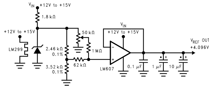
Figure 39. Low Drift Extremely Stable Reference Circuit
