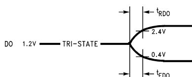
Figure 13. DO “TRI-STATE” Falling and Rising Edge
