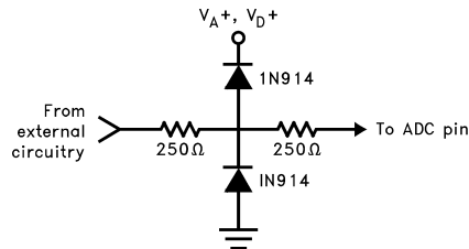
Figure 29. Protecting the MUXOUT1, MUXOUT2, A/DIN1 and A/DIN2 Analog Pins
