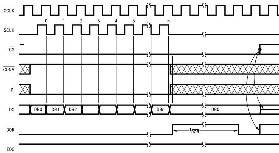
Figure 20. ADC12038 Conversion Using \overline{\text{CS}} with 8-Bit Digital Output Format
