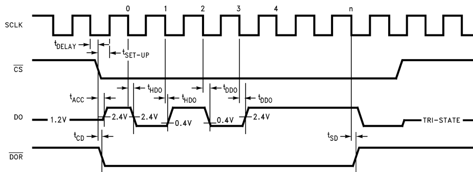
Figure 15. DO Data Output Timing Using \overline{CS}
