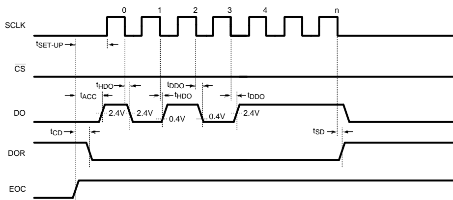
Figure 16. DO Data Output Timing with \overline{\text{CS}} Continuously Low
