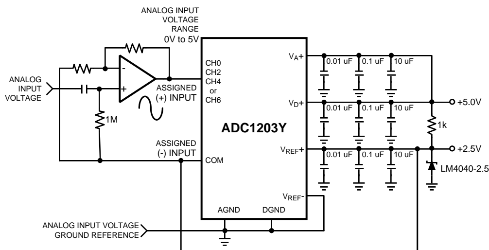
Figure 36. Alternative Pseudo-Differential Biasing
