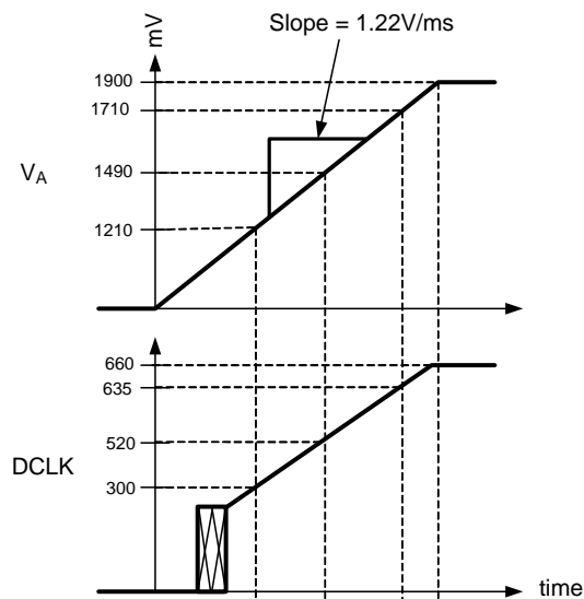
Figure 25. Supply and DCLK Ramping
