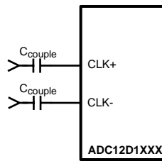
Figure 18. Differential Input Clock Connection
