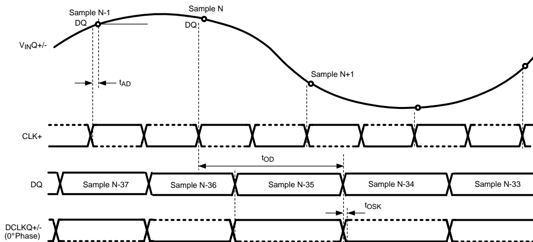
Figure 5. Clocking in 1:2 Demux Non-DES Mode*
