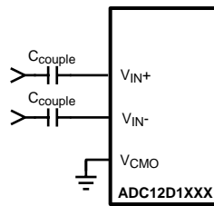
Figure 16. AC-coupled Differential Input
