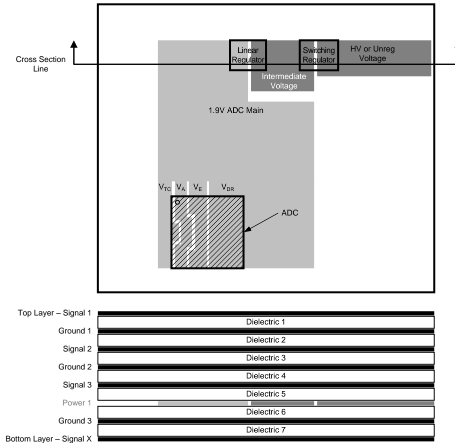
Figure 20. Power and Grounding Example
