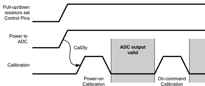
Figure 22. Power-on with Control Pins set by Pull-up/down Resistors
