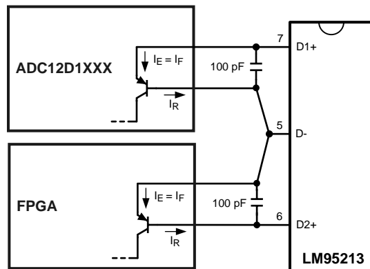
Figure 26. Typical Temperature Sensor Application
