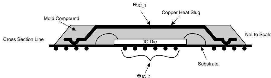
Figure 21. HSBGA Conceptual Drawing
