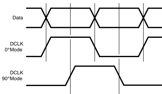
Figure 14. DDR DCLK-to-Data Phase Relationship
