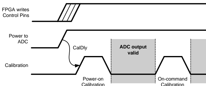
Figure 23. Power-on with Control Pins set by FPGA pre Power-on Cal
