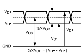
Figure 3. LVDS Output Signal Levels
