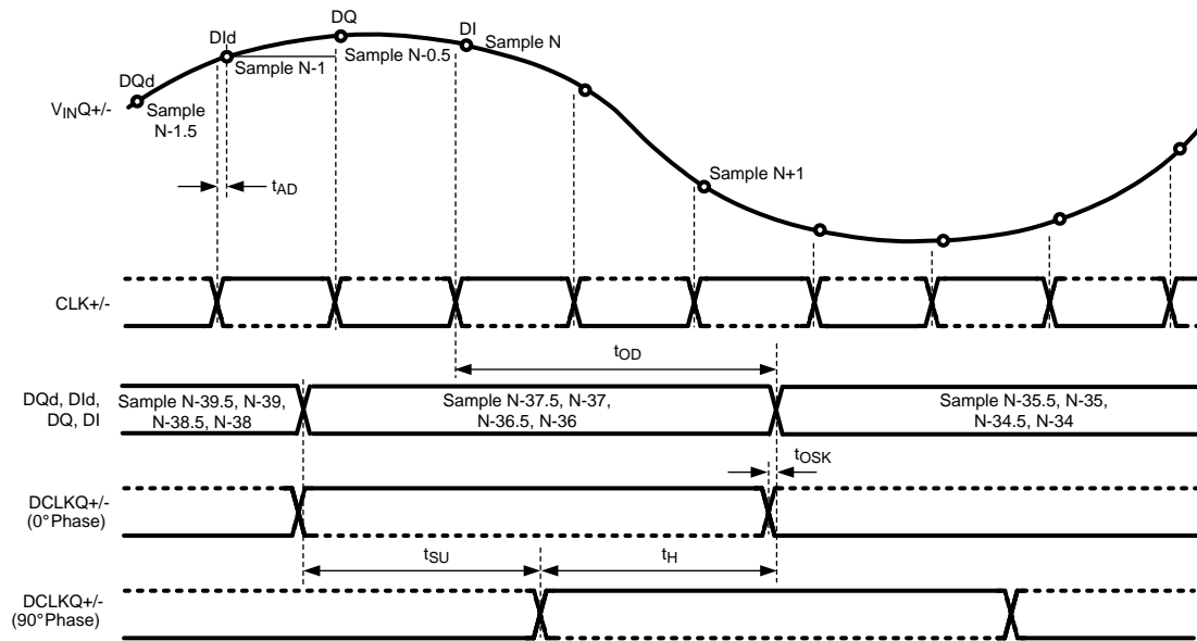
Figure 7. Clocking in 1:4 Demux DES Mode*
