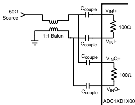
Figure 15. Driving DESIQ Mode
