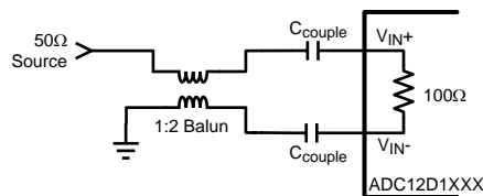
Figure 17. Single-Ended to Differential Conversion Using a Balun
