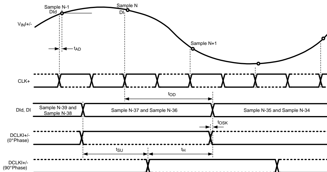
Figure 5. Clocking in 1:2 Demux Non-DES Mode*
