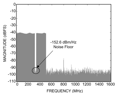
Figure 1. Wideband Performance
