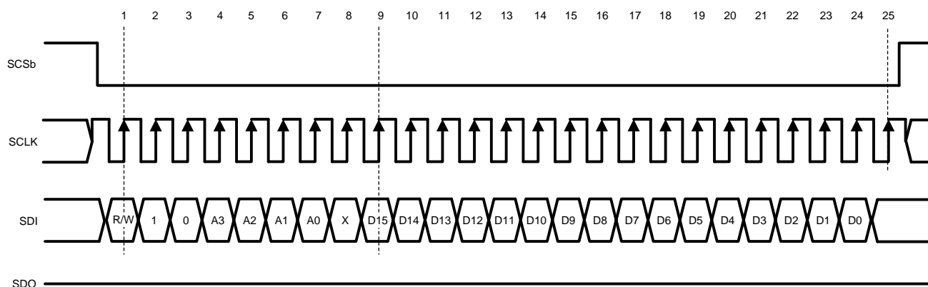
Figure 13. Serial Data Protocol - Write Operation
