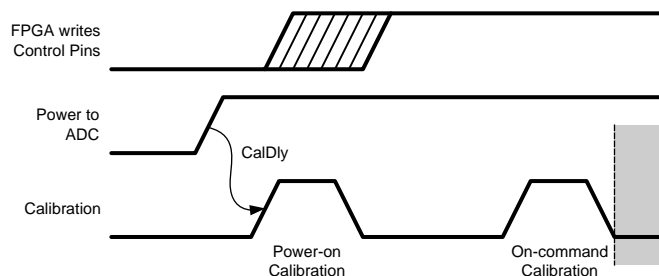
Figure 24. Power-on with Control Pins set by FPGA post Power-on Cal
