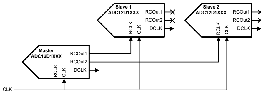
Figure 19. AutoSync Example
