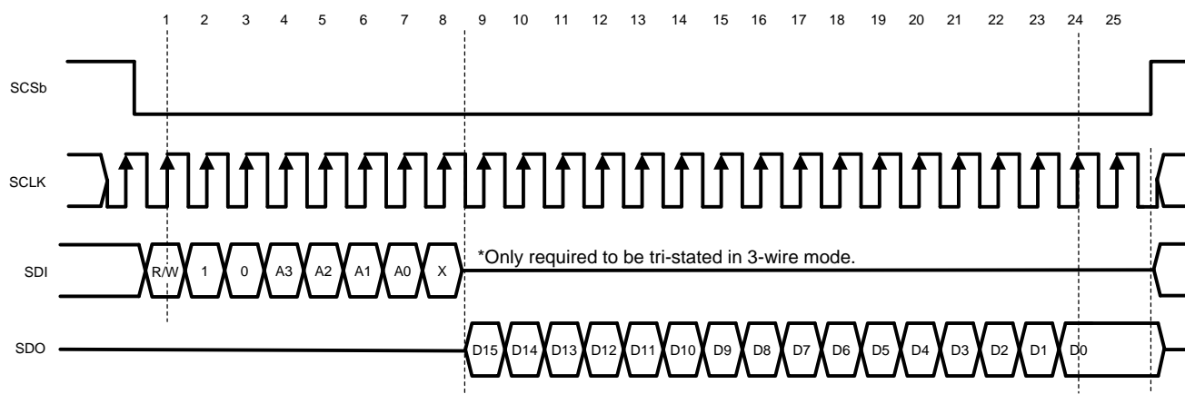
Figure 12. Serial Data Protocol - Read Operation
