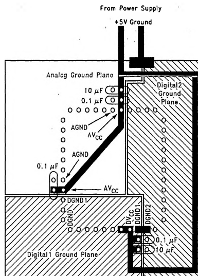
FIGURE 12. PC Board Layout
