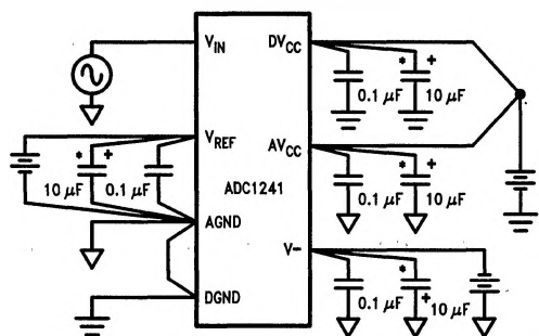
Power Supply Bypassing
