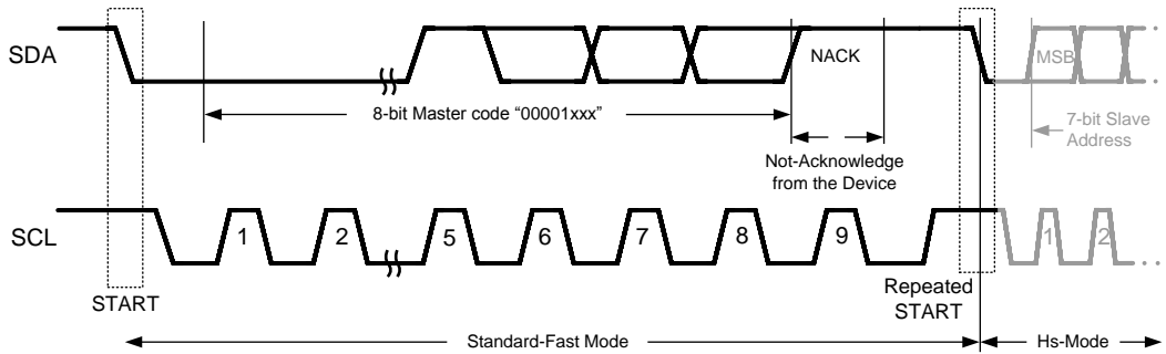
Figure 8. Beginning Hs-Mode Communication
