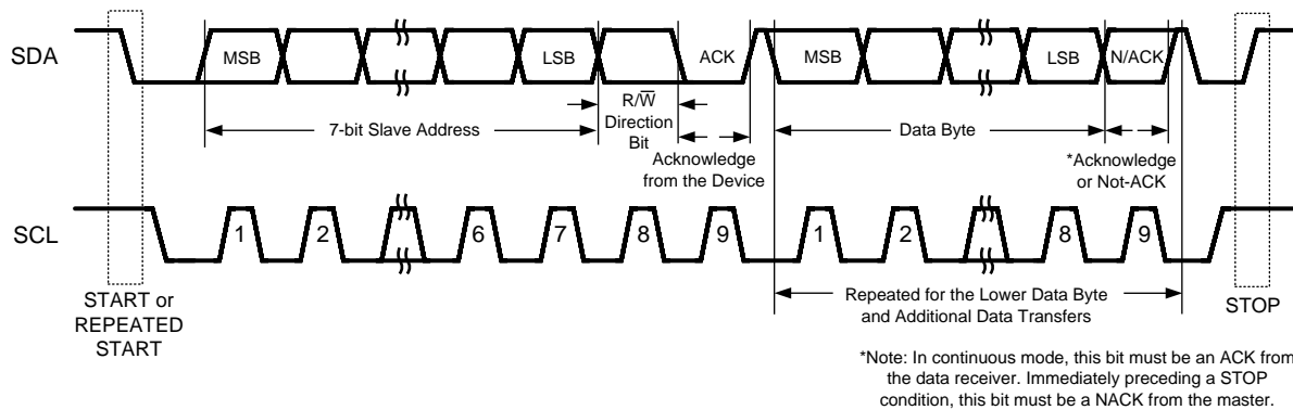
Figure 7. Basic Operation.
