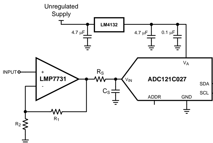
Figure 19. Buffered Input Circuit
