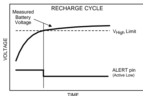
Figure 21. Recharge Cycle
