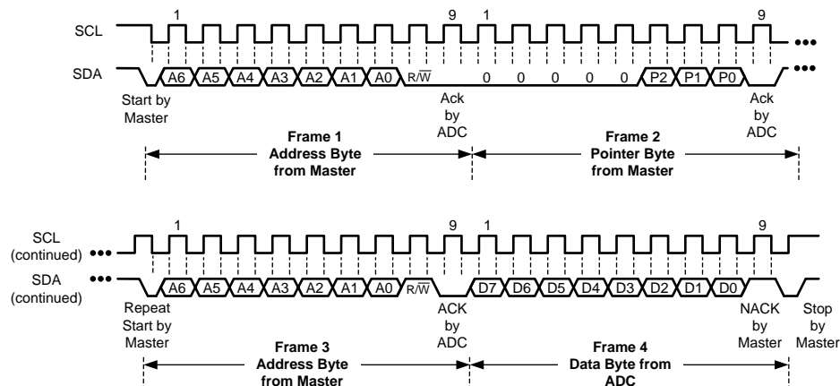
Figure 14. (b) Typical Pointer Set Followed by Immediate Read of a 1-Byte ADC Register
