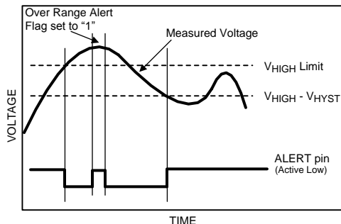
Figure 10. Alert condition cleared by writing a "1" to the Alert Flag.
