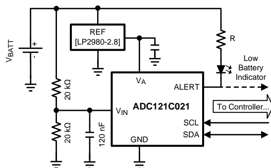
Figure 20. Intelligent Battery Monitor Circuit
