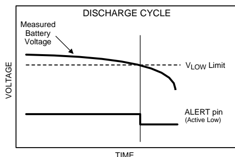
Figure 22. Discharge Cycle
