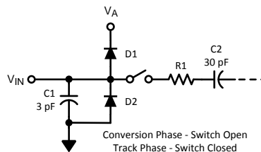
Figure 4. Equivalent Input Circuit
