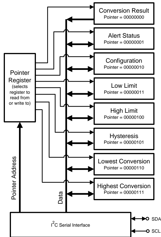
Figure 6. Register Structure
