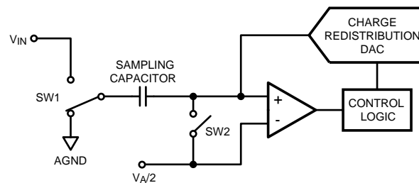
Figure 3. ADC121C021 in Hold Mode
