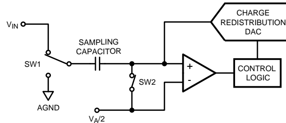
Figure 2. ADC121C021 in Track Mode
