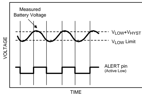
Figure 23. Trickle Charge
