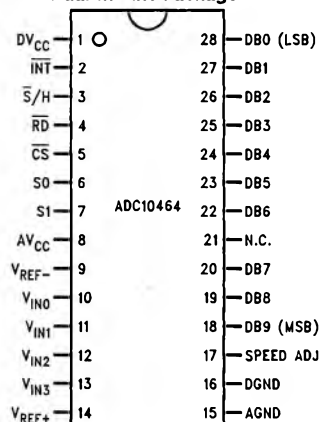
Dual-In-Line Package
