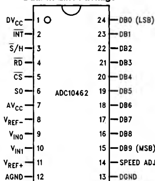
Dual-In-Line Package
