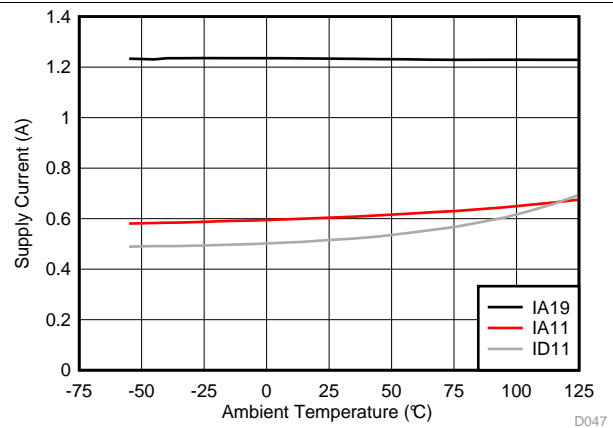
Figure 47. Supply Current vs Temperature
