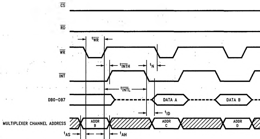
FIGURE 3. WR-RD Mode (Mode Pin is High) Reduced Interface System Connection ( \overline{CS} = \overline{RD} = 0 )
