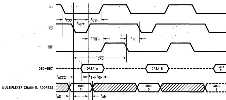
FIGURE 4. RD Mode (Pipeline Operation) (Mode Pin is Low and t_{RDW} must be between 200 ns and 400 ns)
