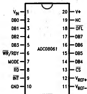
Dual-In-Line and Wide-Body Small-Outline Packages J20A, N20A or M20B
