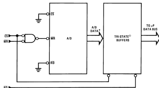
*A/D output data is updated 1 CLK period prior to assertion of \overline{\text{INTR}} Figure 39. Output Buffers with A/D Data Enabled
