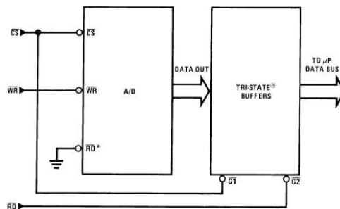
*Allows output data to set-up at falling edge of \overline{\text{CS}} Figure 41. Increasing Bus Drive and/or Reducing Time on Bus
