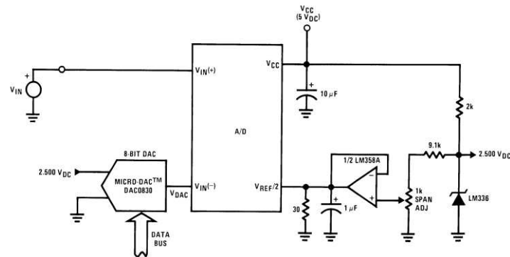
Figure 19. 1 mV Resolution with \mu P Controlled Range
