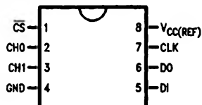
ADC08032 Dual-In-Line Package
