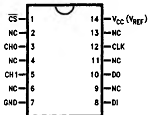
ADC08032 Small Outline Package
