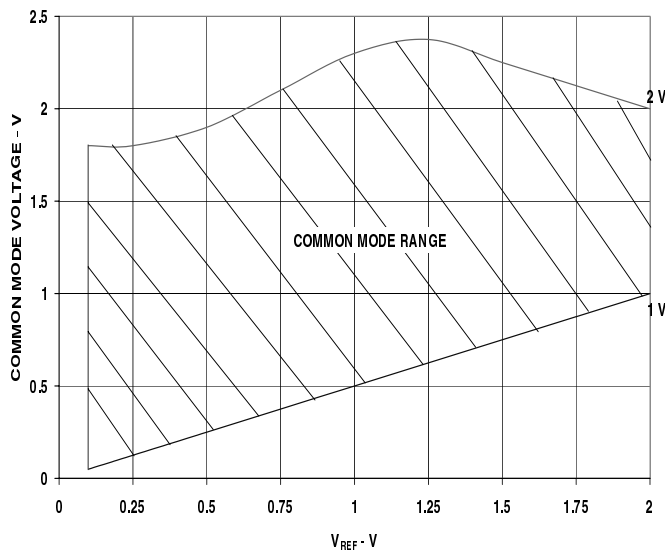
Figure 10. Input Common Mode Range versus V_{REF} ( V_{DD} = 3V and V_{REF(max)} = 2V )
