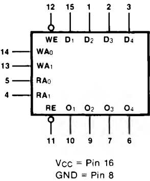
LOGIC SYMBOL
